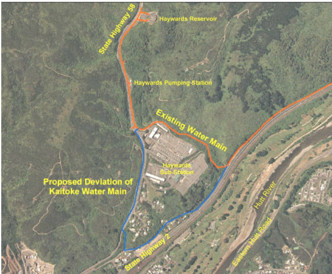
Figure 1 : Existing and proposed diversion of the Kaitoke Main.
