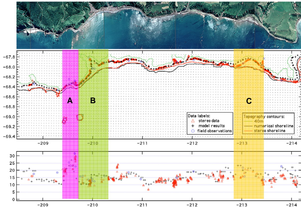
Figure A4 Inundation distance extent and maximum water level for the Okushiri southwest coast, from http://nctr.pmel.noaa.gov/Pdf/photo_graphs_title.pdf , colour bands and labels subsequently added (see text).
