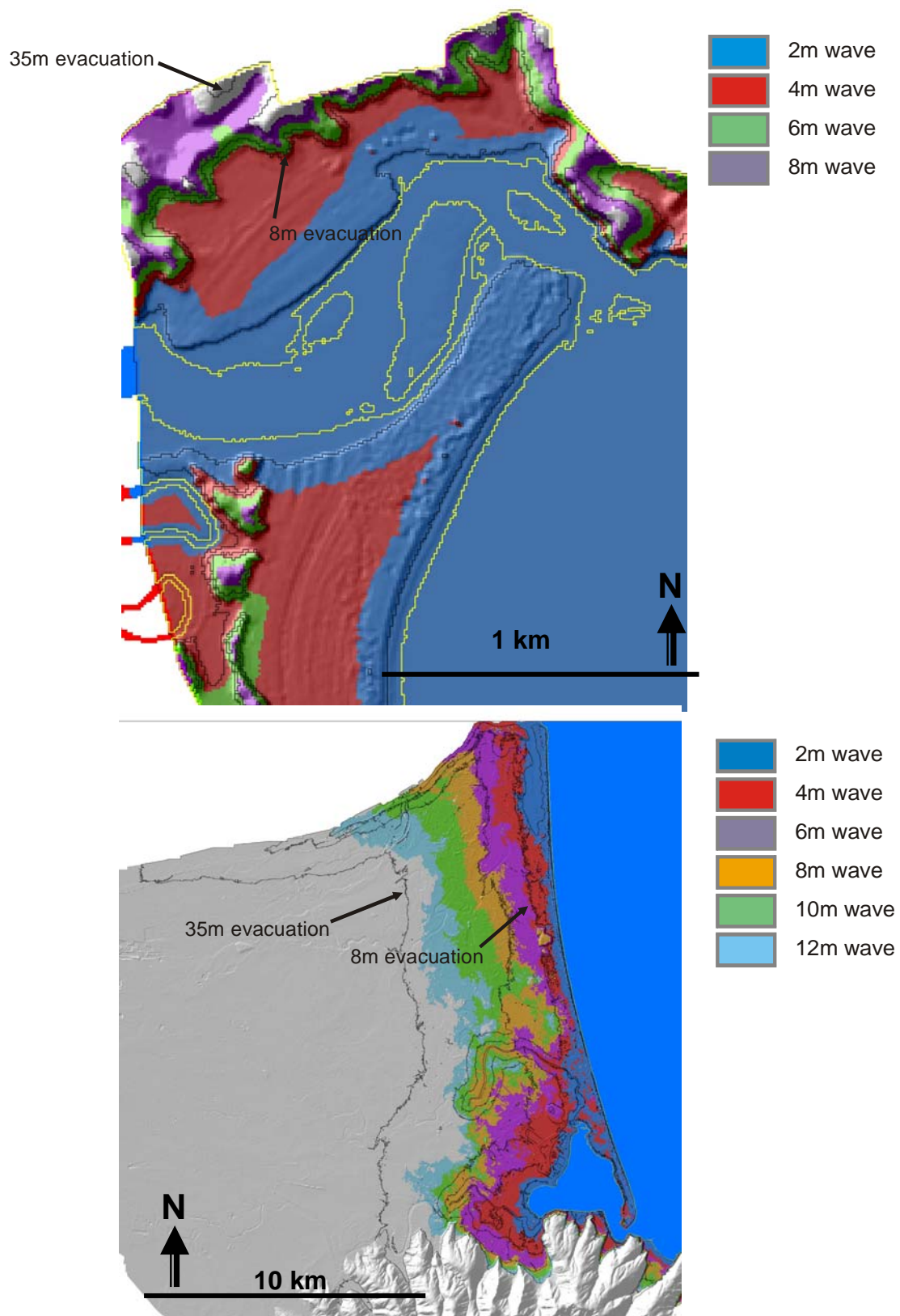
Figure A6 GIS-modelled evacuation zone lines (black, representative lines labelled) compared to Camfield inundation zones (coloured). Top figure is Whananaki, Northland, bottom is Pegasus Bay, Canterbury.
