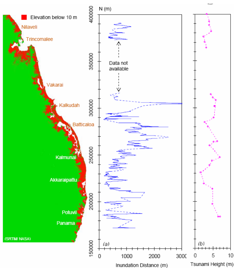
Figure A3 Inundation distance and Tsunami height measurements for the Sri Lanka east coast. From Wijetunge (2006).
