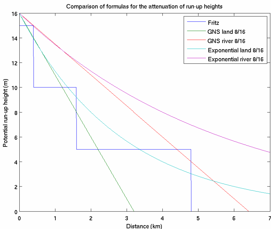
Figure A7 Comparison of Fritz Criteria, linear (used here) and exponential-decay attenuation relationships.
