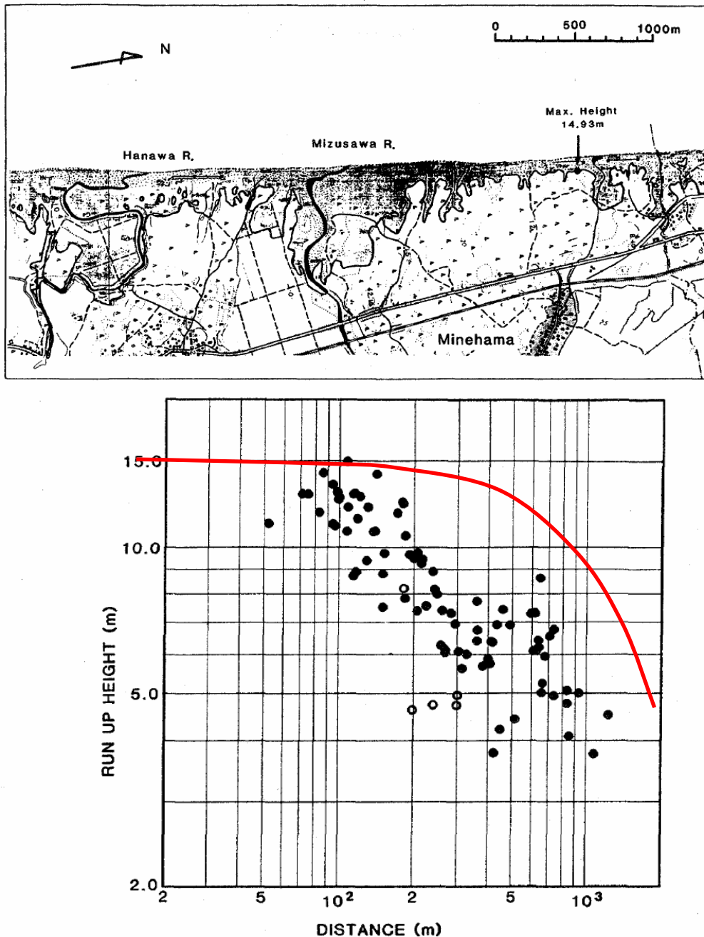
Figure A5 Run-up and inundation heights (m) as a function of the distance (m) from the shoreline on the Minehama coast (Kajiura, 1986). The superimposed red curve illustrates the envelope of points within the 1:200 attenuation curve, assuming a maximum possible run-up at the coast of 15.5m, the enveloped does not appear as a straight line because of the logarithmic scaling of the original plot.
